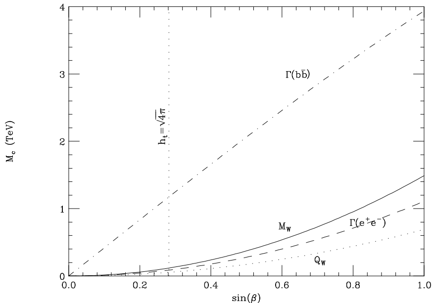
FIG. 1. Bounds on the bulk generations scenario. The h_t line indicates where the top quark Yukawa coupling becomes nonperturbative. The bound from \rho is indistinguishable from the \Gamma(e^+e^-) result.
